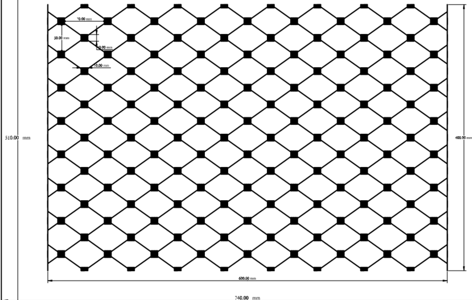
Pattern 154, 50mm x 70mm Single diamond Fill vertical. 12919 stitches.
