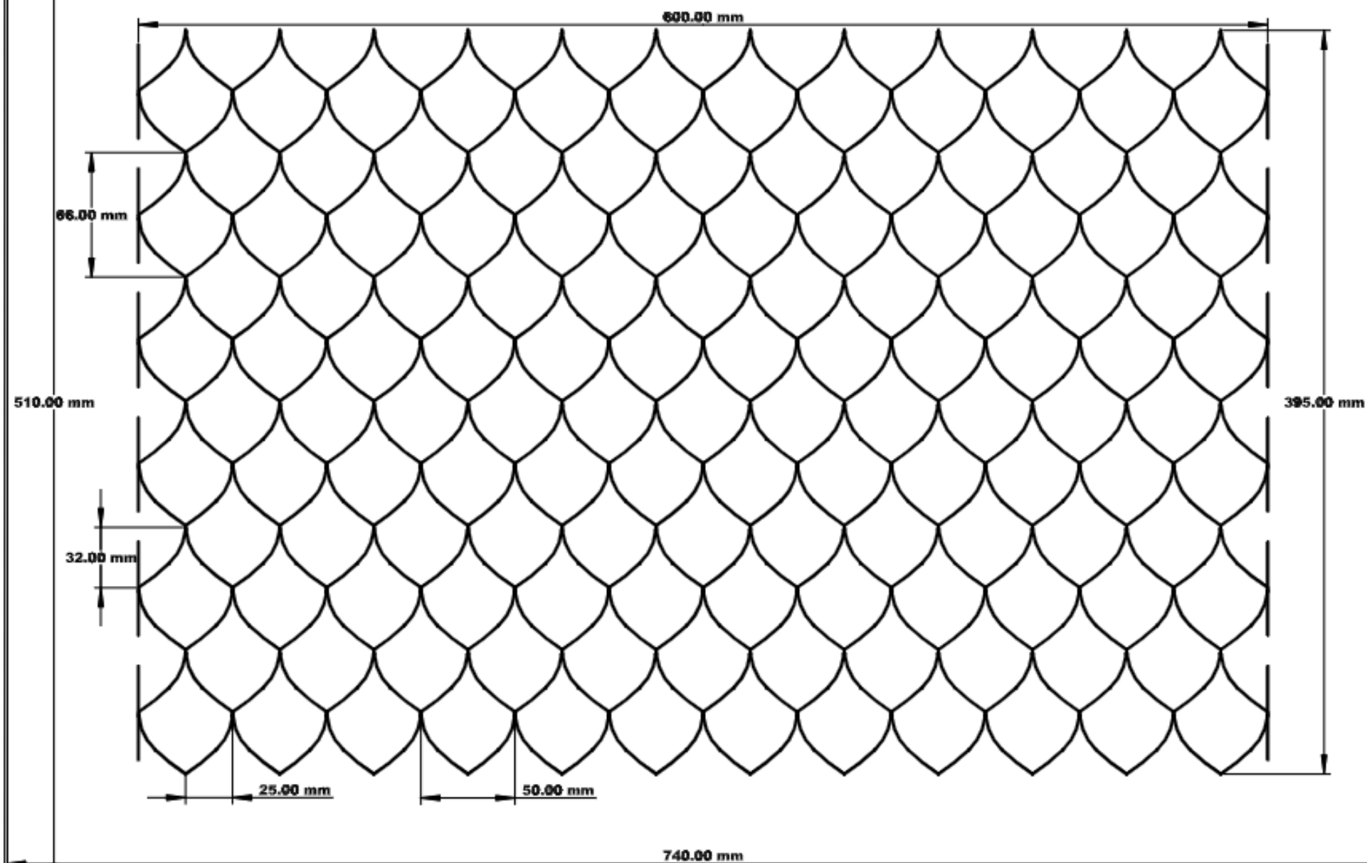
Pattern 135, Scales, Horizontal. 3120 Stitches.
