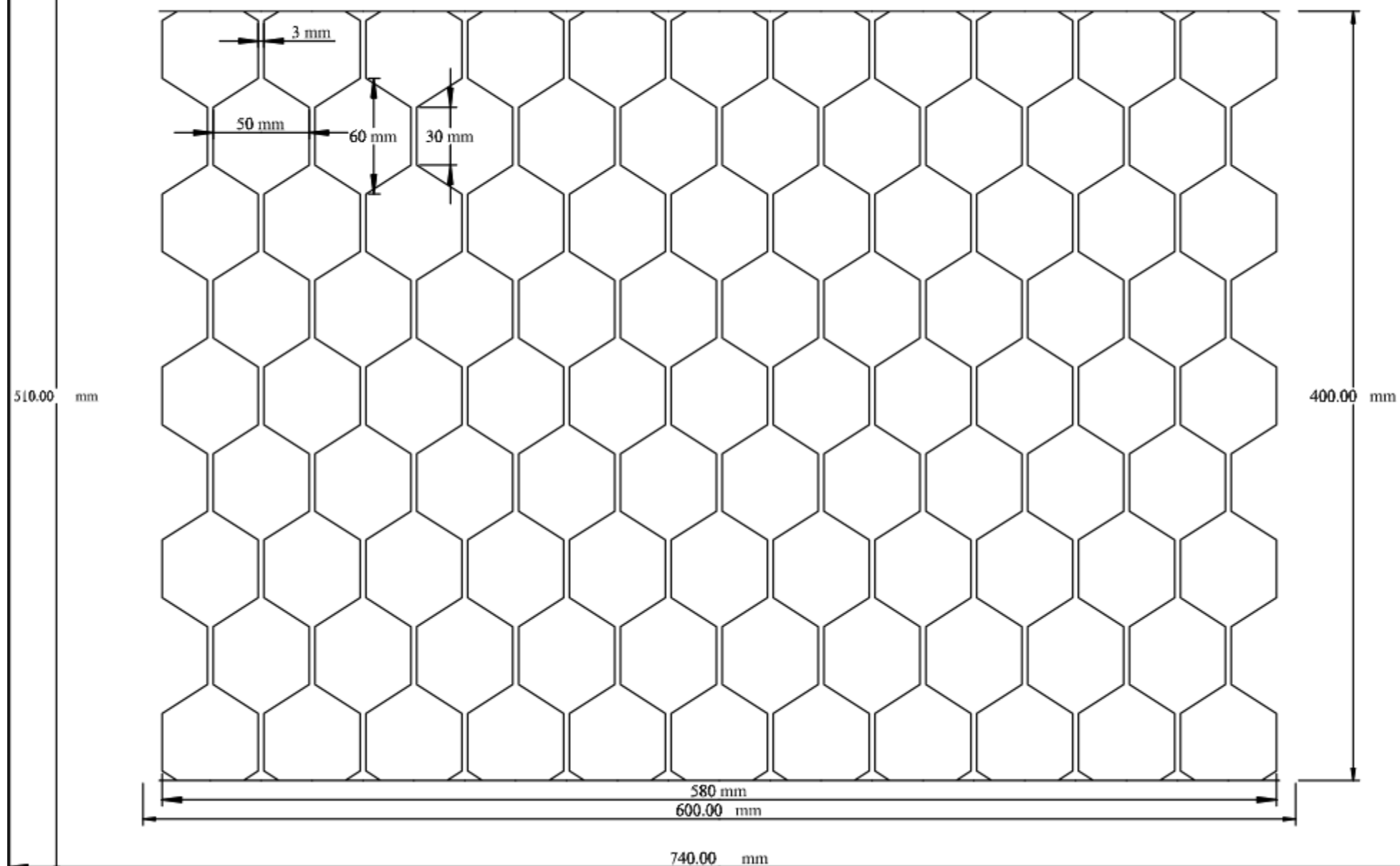
Pattern 230, 50mm Hexagonals Vertical. 4378 Stitches.
