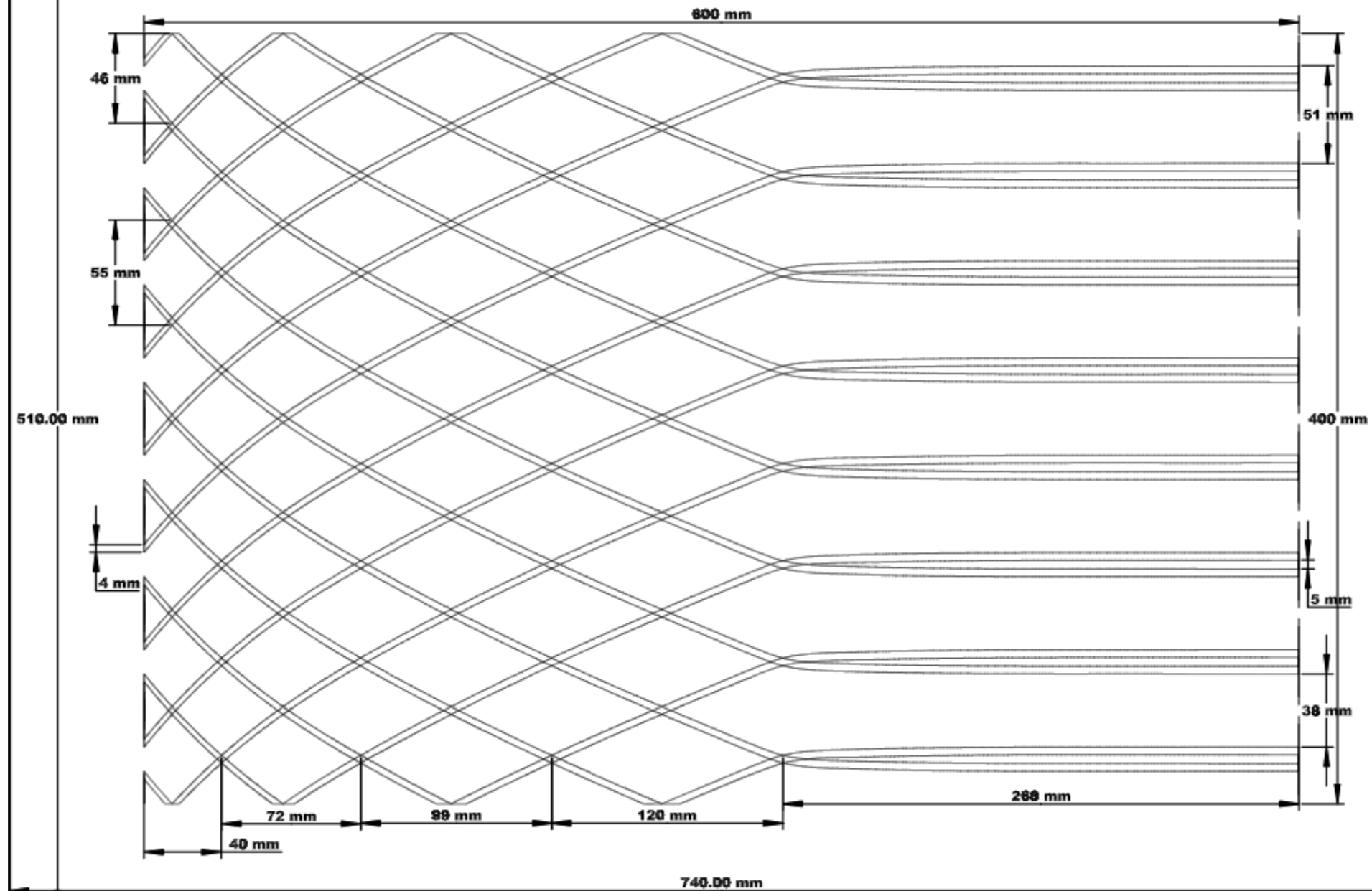
Pattern 138, Reticulated pinstripe diamonds. 7184
