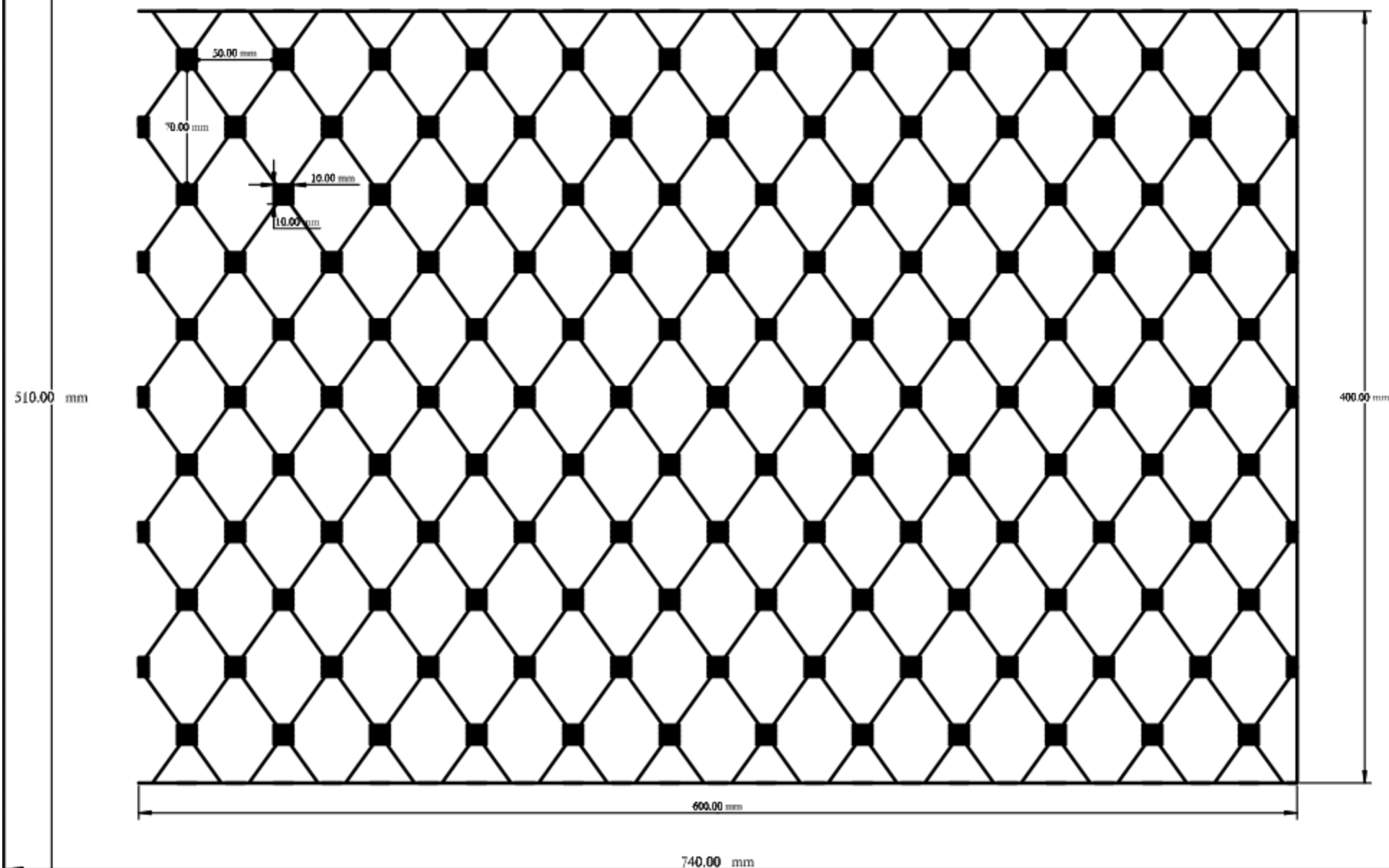
Pattern 155, 50mm x70mm diamond fill Horizontal. 12919 Stitches.
