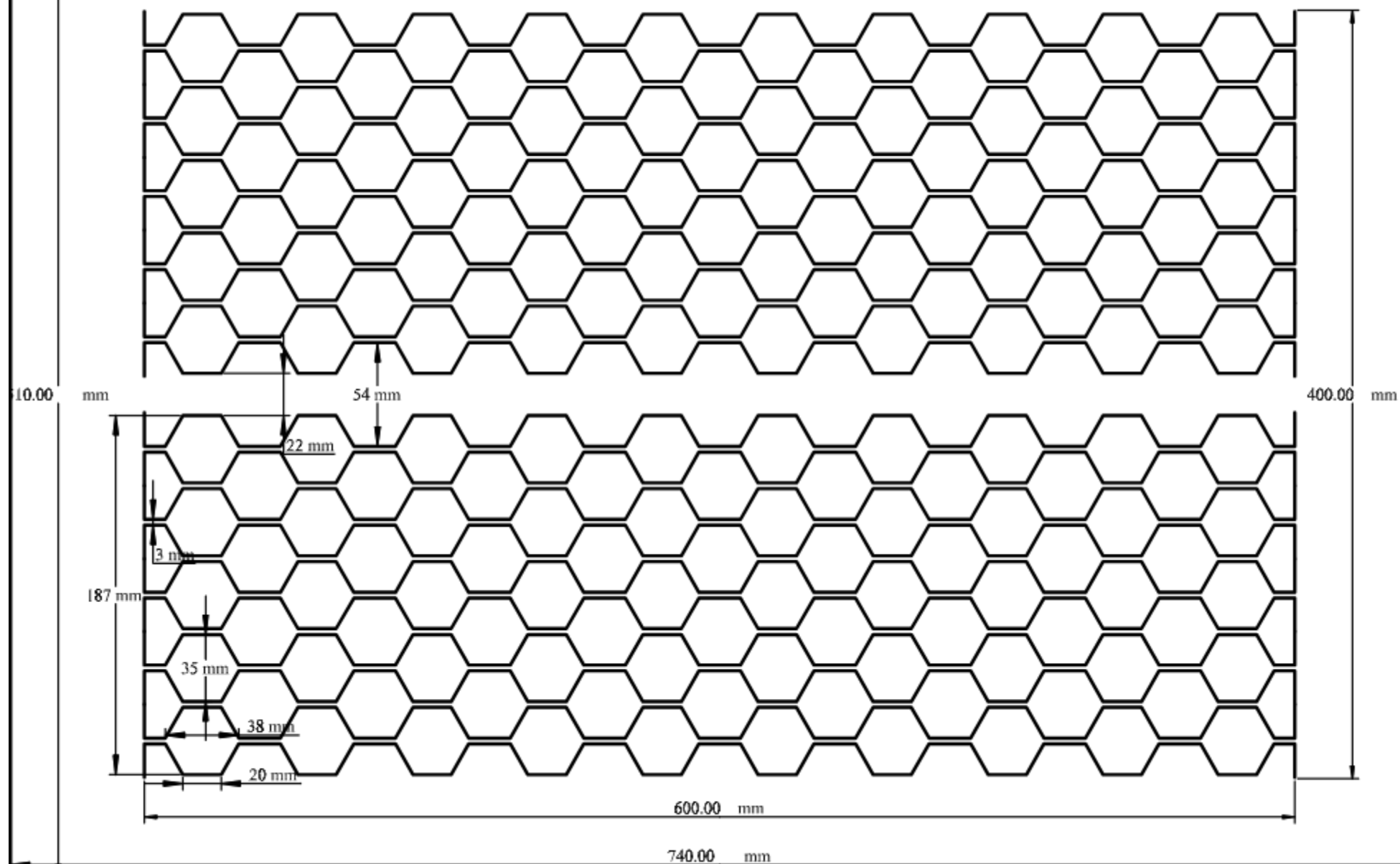
Pattern 239, Hexagonals verticals x 2. 4340 stitches.
